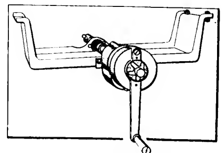
Fig. 3—The Hartford safety crank to overcome the deleterious effects of backfires
